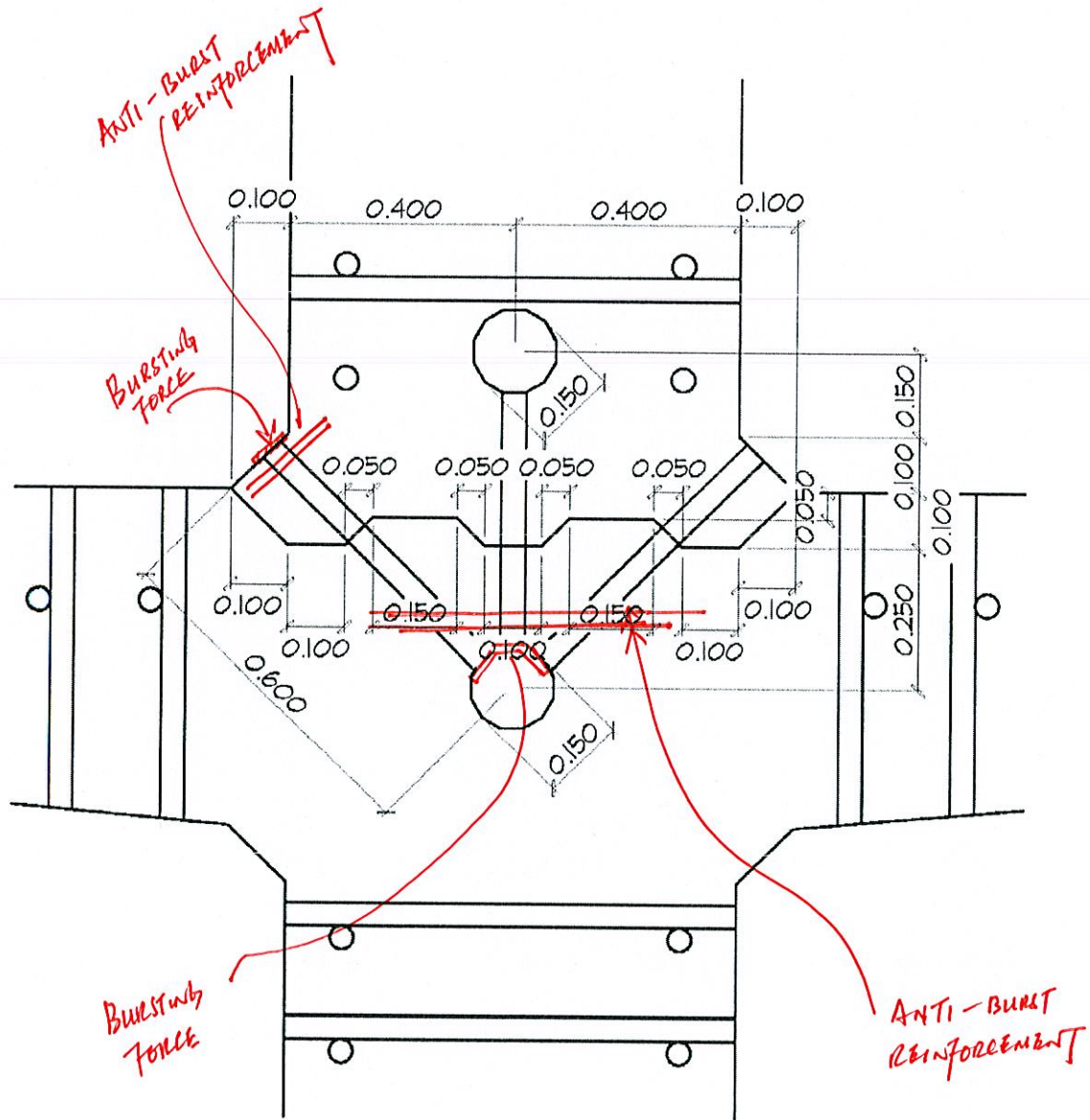
FIGURE 6.1.2.4 TYPICAL COLUMN BASE CONNECTION INFO.
