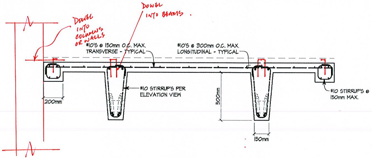
FIG. 6.3.3 (B) FLOOR PANEL SECTION AT MIDSPAN SHOWING REINFORCING
